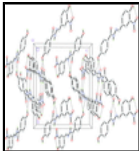
Fig. 2. A perspective view along the a-axis of the crystal packing of the title compound. The hydrogen bonds are shown as dashed lines. H-atoms not involved in hydrogen bonding have been omitted for clarity.
